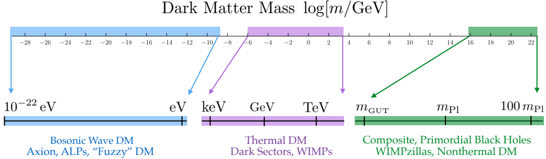
FIG. 1. Range of available dark matter candidates. Current observations allow for dark matter to consist of quanta with an enormous range of masses. Here we classify these candidates as particle-like when m \gtrsim 1 eV, and ultralight, wave-like dark matter when m \lesssim 1 eV. A few prototypical models are listed as examples.
