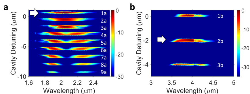
Figure 2: Measured output spectra as a function of cavity lengths for the a , 2- \mu\text{m} OPO and b , 4- \mu\text{m} OPO. The white arrows show the cavity lengths for stable half-harmonic generation.
